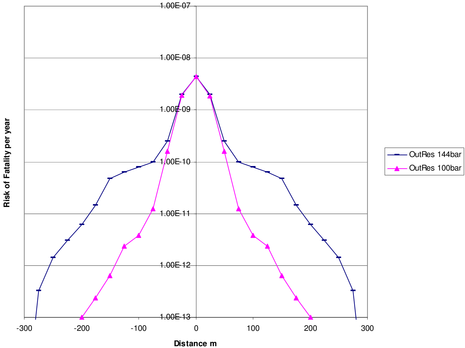
Risk Transects Corrib Pipeline - Person outdoors for 8 hours per day IGE
